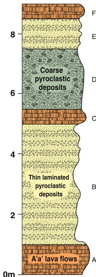
Fig. 12.10 Schematic stratigraphic column of the Las Calvas del Teide area: volcaniclastic deposits (B, D, E) are intercalated with phonolitic lava flows of “Old” Teide (A, C, F) (modified from Pérez-Torrado et al. 2004)
