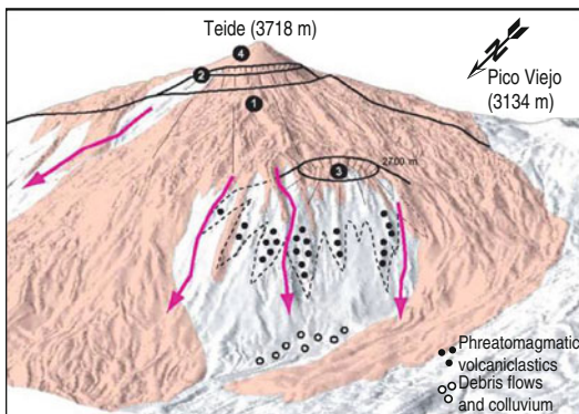
Fig. 12.9 Outcrops of the volcaniclastic and associated deposits from the Las Calvas del Teide phreatomagmatic eruption. 1 Lavas Negras (ca. 1.2 ka). 2 "Old" Teide (>30 ka). 3 Las Calvas del Teide inferred phreatomagmatic vent. 4 Summit cone of the Las Calvas del Teide eruption
