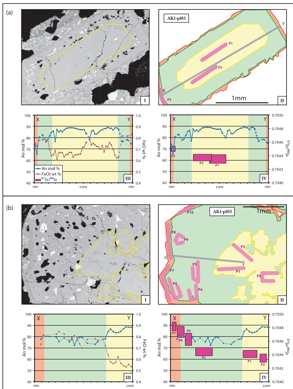
Fig. 8. Examples of plagioclase crystals broadly indicating AFC-type processes: (a) phenocryst AK1-pl01; (b) phenocryst AK1-pl03; (c) phenocryst AK1-pl04; (d) phenocryst AK1-pl09. Each section of (a)–(d) is split into four parts: part I, a back-scattered electron image to illustrate the plagioclase troughs; part II, a graphic representation of the plagioclase zones and the position of the ^{87}\text{Sr}/^{86}\text{Sr} LA-ICP-MS analyses and the EMP traverse (labelled X–Y); part III, An mol % (diamonds) and FeO wt % (circles) zoning profile from X to Y; part IV, An mol % profile plotted against ^{87}\text{Sr}/^{86}\text{Sr} (bars). In part IV, the length and height of the rectangles corresponds to the lasered area and analytical error (2SD), respectively.
