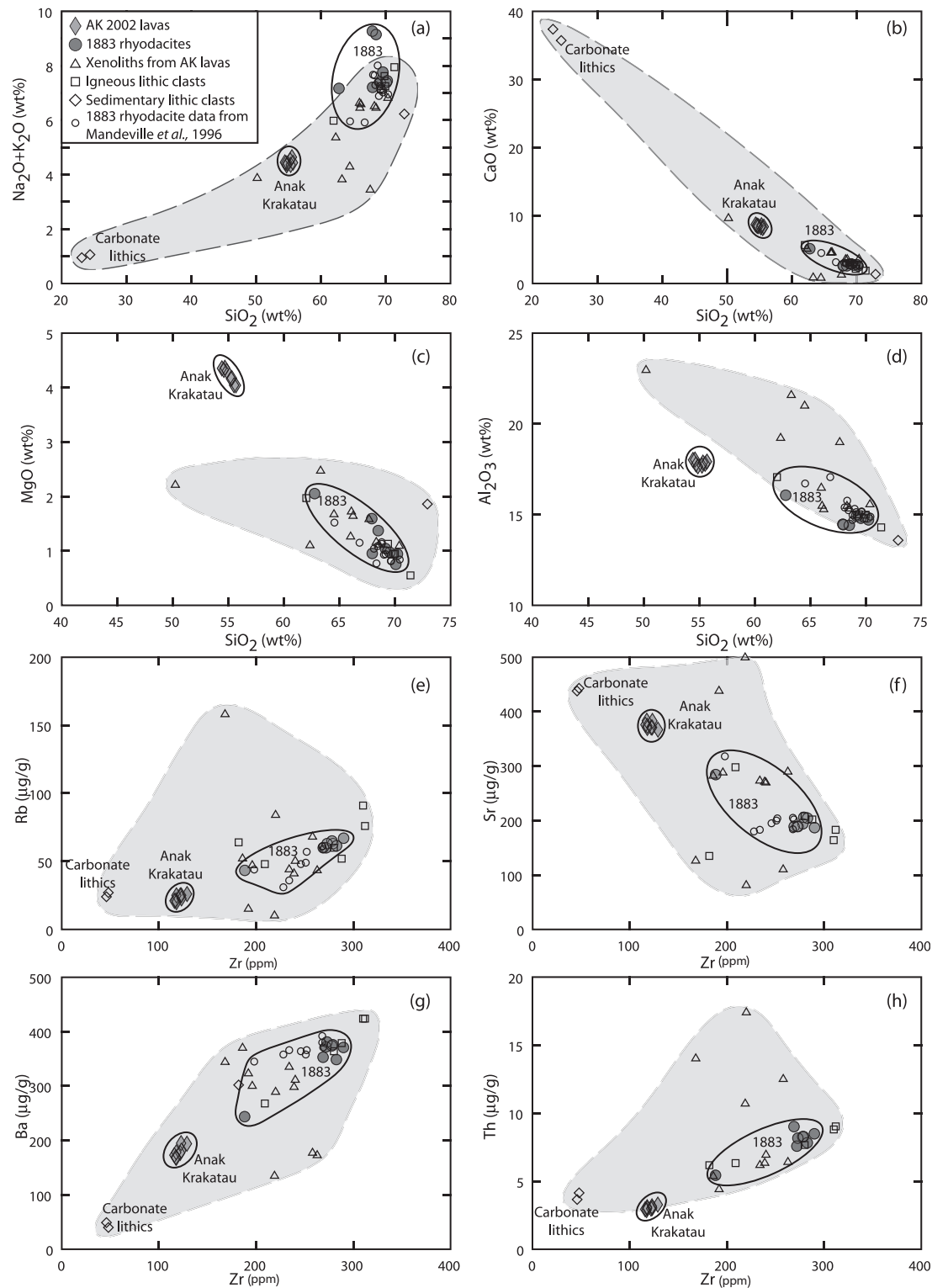
Fig. 4. Major and trace element variations for Anak Krakatau, 1883 and related samples. Major oxides are plotted against \text{SiO}_2 (concentrations in wt %) and trace elements against Zr (in ppm). Xenoliths (e.g. metasedimentary and igneous clasts) are also shown [note the different scale in (c) and (d) when the carbonate lithics are not plotted]. Data from Mandeville et al. (1996) are also included as small open circles. The fields outlined with dashed and continuous lines denote the range of Anak Krakatau basaltic andesites and in the composition of the 1883 eruption products, respectively. The grey field defines the entire range of possible contaminants, defined by lithic clasts from within the 1883 deposits and xenoliths from the Anak Krakatau lavas.
