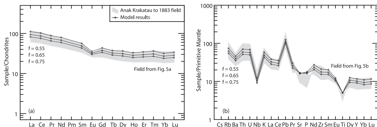
Fig. 10. Fractional crystallization models for 25%, 35% and 45% crystallization (fraction of remaining liquid, f = 0.75 ; 0.65 and 0.55 ) shown as (a) chondrite-normalized REE patterns and (b) primitive mantle-normalized multi-element patterns (shaded area is the field bounded by Anak Krakatau basaltic andesites and 1883 rhyodacites as shown in Fig. 5a and b).
