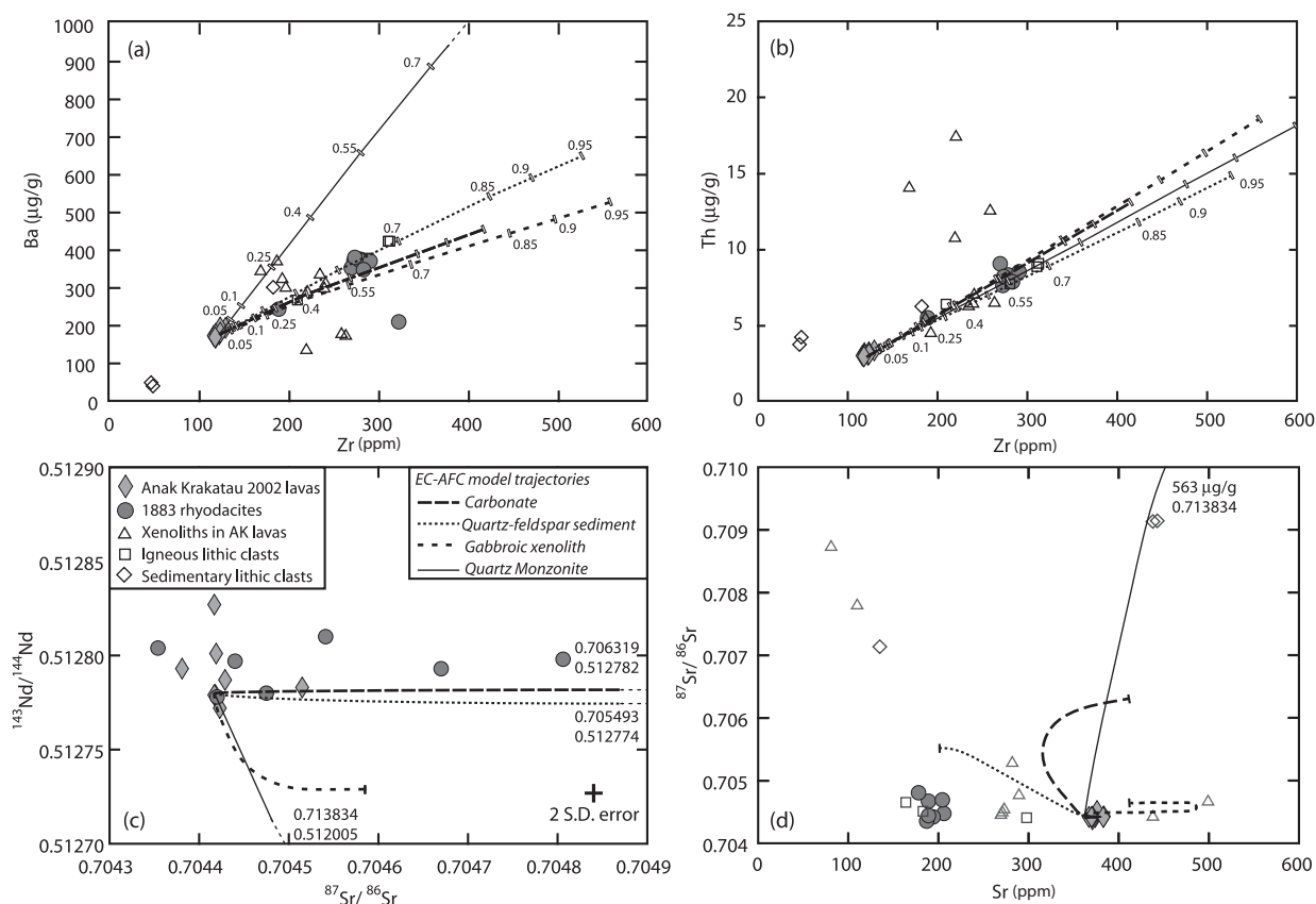
Fig. 11. Simple assimilation and fractional crystallization (AFC) models showing (a) Ba vs Zr and (b) Th vs Zr (in ppm) for increments of f (where f is fraction of remaining liquid). The model results plotted are representative of all trace elements investigated. Four possible contaminants are modelled, a carbonate (long-dash line, sample K.S.SC-05/06), a quartz-feldspathic sediment (dotted line, sample K.S.SC-07), a gabbroic xenolith (short-dash line, sample AK.Xla-05 x) and a hypothetical quartz monzonite (continuous line). Only results for r = 0.3 are shown for ease of correlation. Results from energy-constrained assimilation and fractional crystallization simulations (EC-AFC) are shown in (c) for ^{143}\text{Nd}/^{144}\text{Nd} vs ^{87}\text{Sr}/^{86}\text{Sr} and (d) for ^{87}\text{Sr}/^{86}\text{Sr} vs Sr concentration (ppm). Trajectories of projected magma compositions are plotted for each of the four considered assimilants, with dashed lines and equilibrium compositional values marked if the trajectory extends off the diagram.
