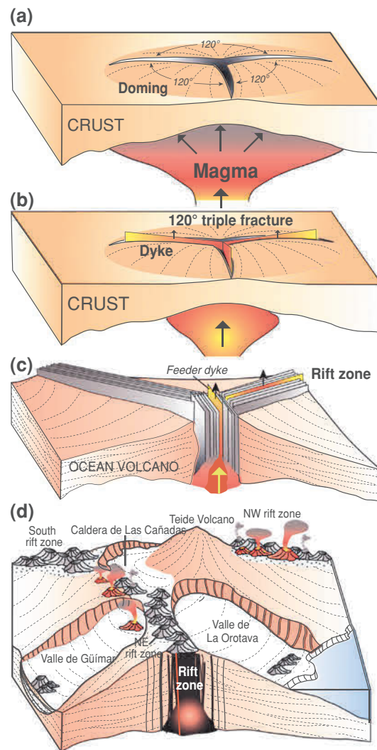
Fig. 4.6 Model proposed by Carracedo (1994, 1996) linking volcanic rift zones and landsliding in the Canary Islands. Three-armed rifts, spaced at \sim 120^\circ , seem to be the naturally preferred configuration, as in the case of El Hierro and Tenerife. This architecture is thought to be a response to least-effort fracturing. The resulting three-sided base pyramidal edifice geometry may be further enhanced by landsliding between the rift arms, propagating perpendicular to the rift direction
