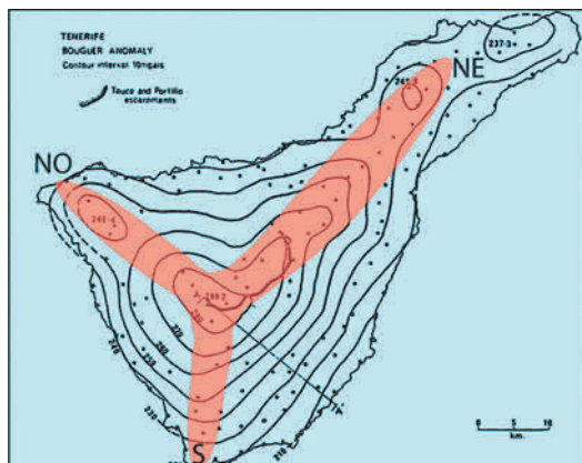
Fig. 4.3 Bouguer anomaly map of Tenerife showing a three-pointed star shape (from MacFarlane and Ridley 1968)
