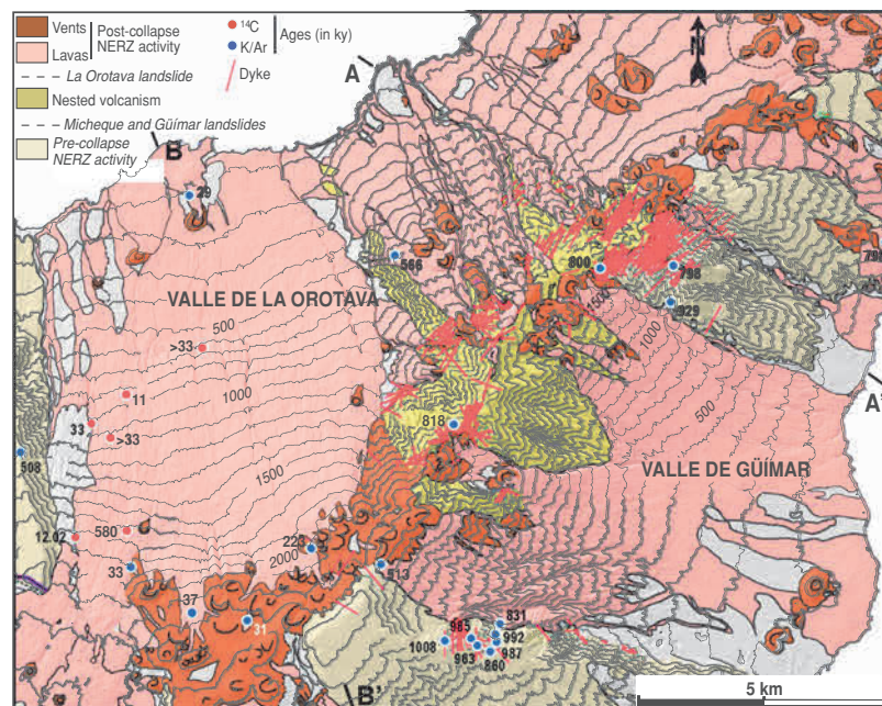
Fig. 4.12 Simplified geological map of the NE Rift Zone of Tenerife showing the distribution of eruptive vents and lava flows. Ages (in ky) from Carracedo et al. (2011)
