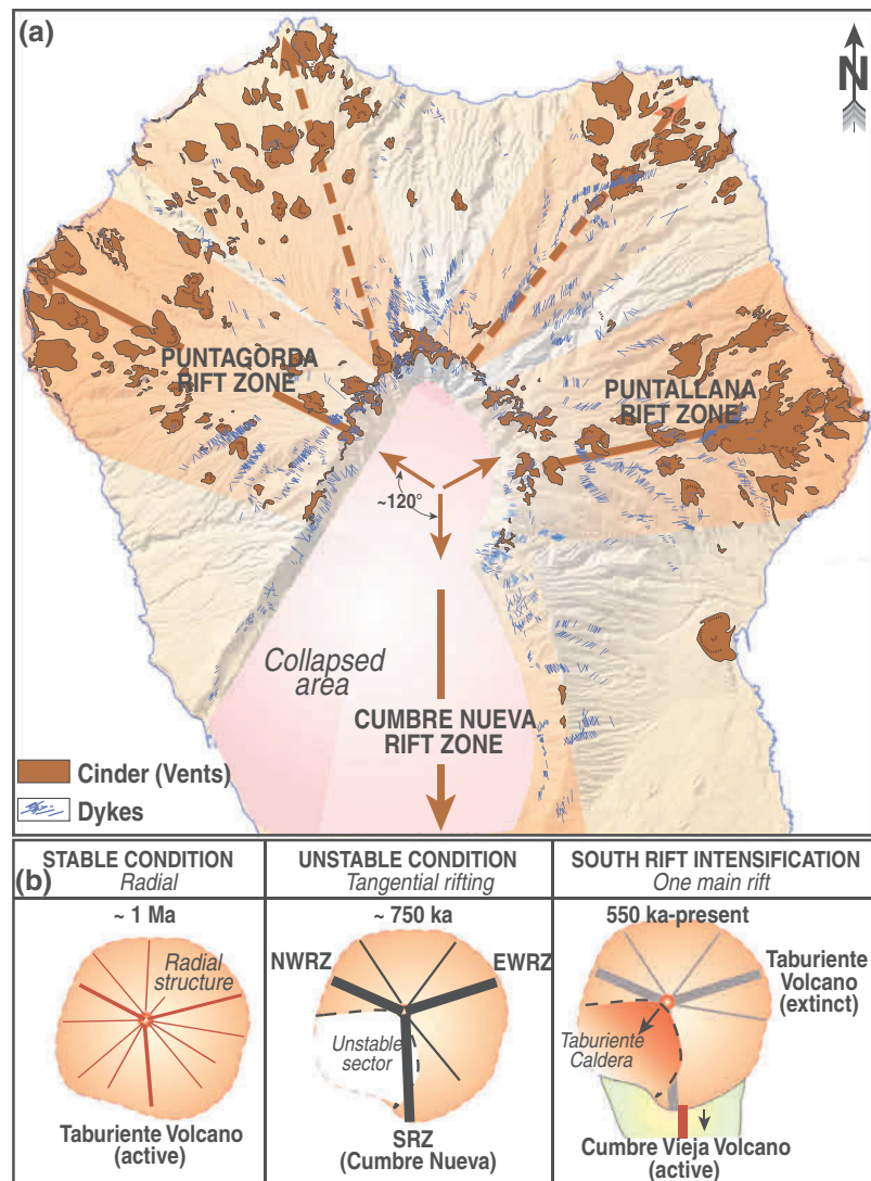
Fig. 4.8 a Eruptive vents and dyke outcrops of the Taburiente shield volcano ( \sim 0.77 – 0.4 Ma), La Palma, with rift zones forming a radial structure. The incipient three-armed rift organisation ( solid lines ) was apparently left incomplete by the extinction of Taburiente Volcano at an early stage of development (from Carracedo et al. 2001). b Stages of structural evolution of La Palma from an initial radial structure. The position and direction of the creeping flank favoured extension in an east–west direction on the southern flank, and thus the formation of a north–south rift zone. Once formed, the main south rift stabilized by the alternation of constructive and destructive processes such as volcanism, landsliding and erosion (modified from Walter and Troll 2003)
